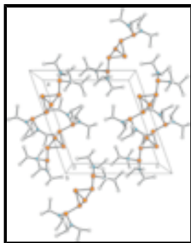
Fig. 2. Packing diagram for 1 . View direction is parallel to the crystallographic b axis.
