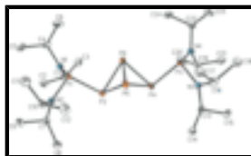
Fig. 1. A view of the molecule of 1 , showing the atom-labelling scheme. Displacement ellipsoids are drawn at the 30% probability level and H atoms have been omitted.
